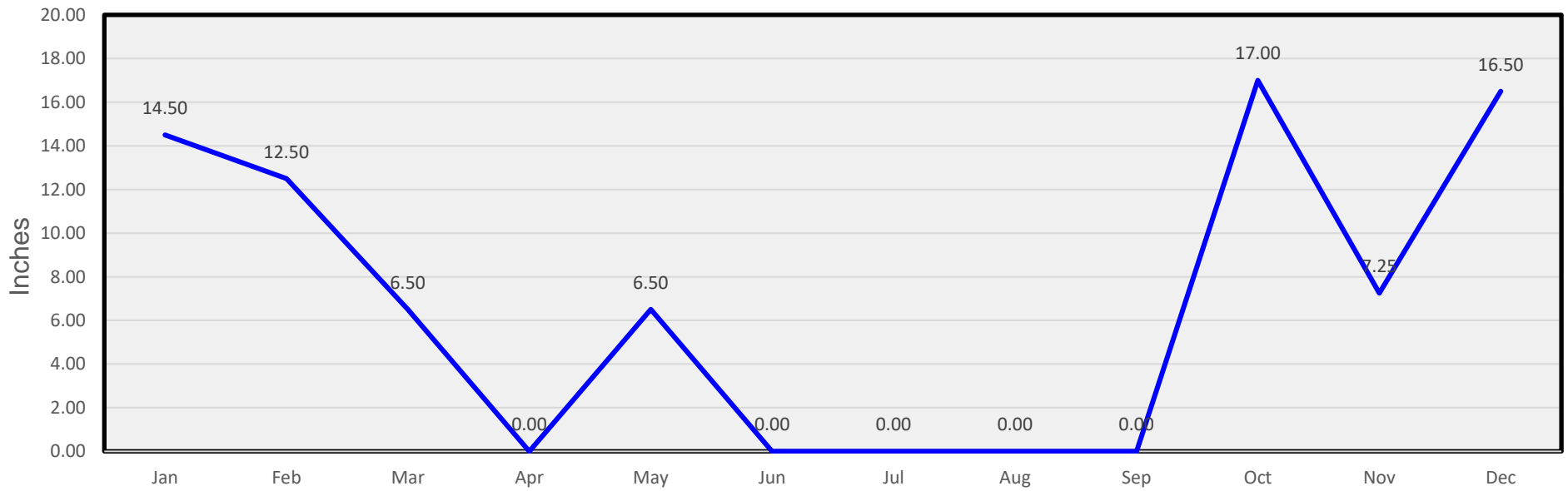
Monthly Snow
