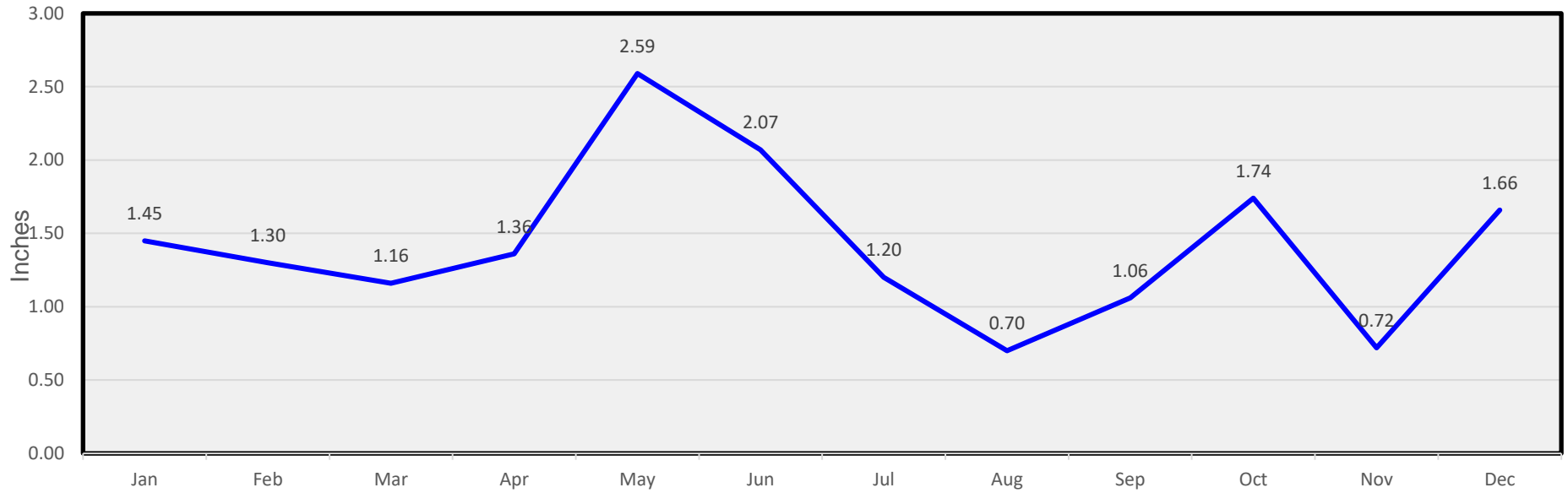
Monthly Precipitation
