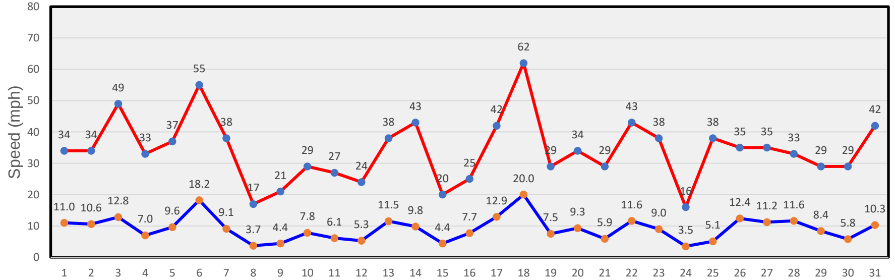
March Winds
