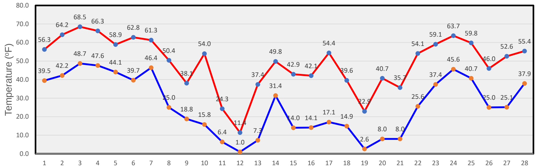
February Temperatures
