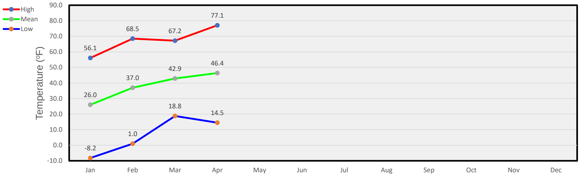
Monthly Temperatures
