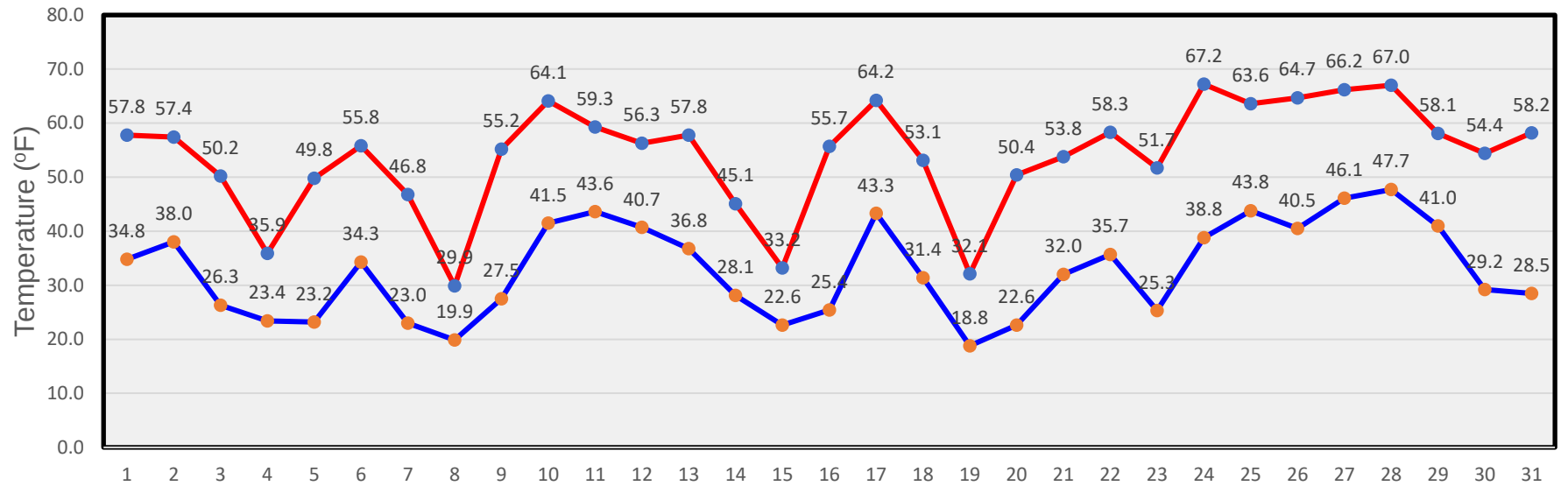
March Temperatures
