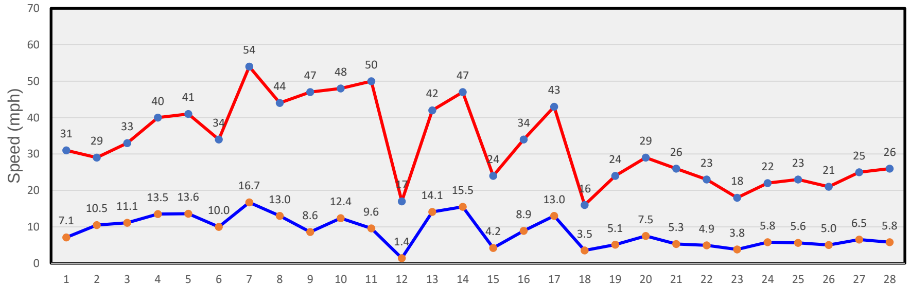
February Winds
